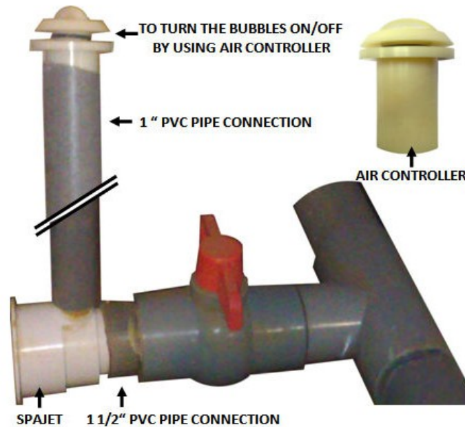
INSTALLATION SAMPLE
